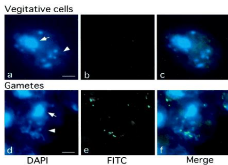
Fig.1 Methylation of chloroplast DNA visualized by immunocytochemistry. Samples are Chlamidomonas me-1 cells.
