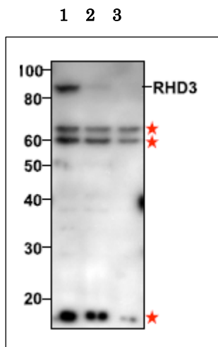
Fig. Validation of anti-RHD3 antibody with mutant plants
